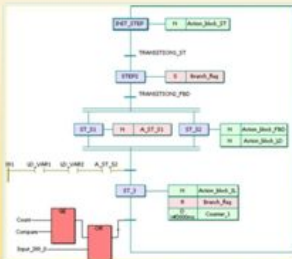
Sequential Function Chart (SFC)
