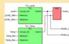
Function Block (FB)
